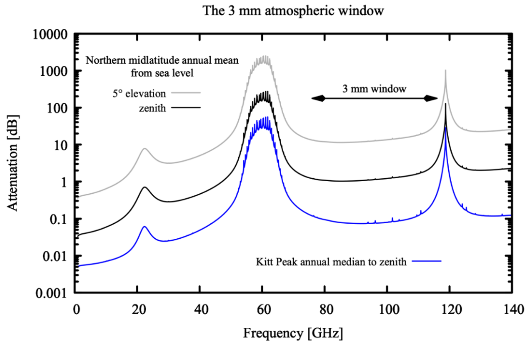
FIGURE 1 Clear sky atmospheric attenuation from sea level to zenith and for a slant path at 5 degrees elevation for a mean annual northern midlatitude atmosphere. Also shown is the median annual zenith attenuation from a representative millimeter-wave observatory site, Kitt Peak, Arizona. Note that the 3 mm atmospheric window is quite transparent even from sea level, with only 1 dB of attenuation towards zenith (radio astronomy) or towards the nadir (Earth remote sensing). Transmissions from aircraft, even at long slant-paths associated with low elevations, are particularly problematic due to their long horizon distances and relatively modest atmospheric attenuation at these frequencies. For this figure and those below, climatological data are from the NASA MERRA-2 reanalysis 6 and attenuation is computed with am-11.0.
