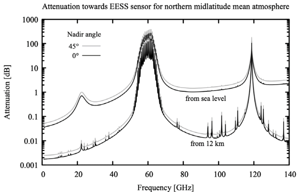
FIGURE 3 Clear sky atmospheric attenuation for two different geometries (45 degree and 0 degree nadir angle) and two different transmitter locations (sea level (ground-based) and 12 km altitude (i.e., aircraft)), for mean northern midlatitude conditions. Note the low atmospheric attenuation at 86-92 GHz, the frequency band allocated to EESS (passive), which is adjacent to the bands under discussion in this NPRM. Out-of-band and spurious emissions into the adjacent passive band from uplinks and aircraft-to-aircraft transmissions in the 80/90 GHz bands will corrupt these critical EESS measurements.
