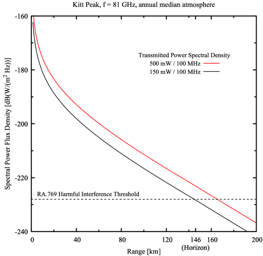
FIGURE 2 Illustration of the sensitivity of radio astronomy observatories at 81 GHz to human-made emissions expressed in terms of the signal strength received at an observatory as a function of separation distance for two different transmitted power spectral densities, accounting for free space loss and atmospheric attenuation. Under atmospheric conditions common to sites of millimeter-wave radio telescopes (illustrated here for the Kitt Peak 12m telescope), separation distances of hundreds of kilometers are required between radio astronomy observatories and ground-based transmitting devices. US Footnote 161 designates coordination zones of 150 km around each single-dish millimeter-wave radio astronomy observatory within the United States. While these sites do experience times of higher atmospheric attenuation in moist weather, median weather conditions at Kitt Peak, Arizona, require separation distances of 150 km for isotropic transmitters of 150 mW/100 MHz due to the sensitivity of radio telescopes designed to detect faint cosmic sources. Increasing the power level to 500 mW/100 MHz would substantially impact radio astronomy observatories by exceeding the ITU-R RA.769 threshold levels for harmful interference when transmitting outside of the US161 coordination zones.
