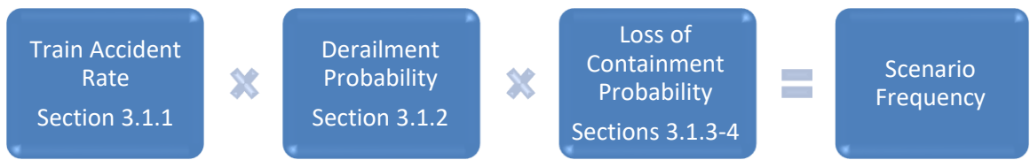
Figure E1. LNG DOT-113 train accident model overview.
