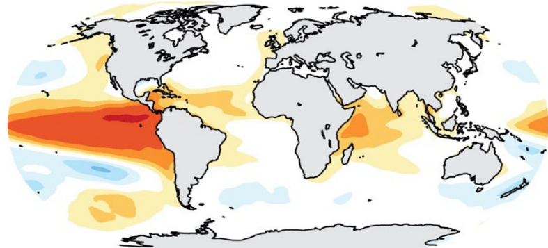
(a) CMIP5
