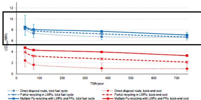
LCOE Fuel cycle for different reactor fleets and back-end strategies (3% discount rate)
