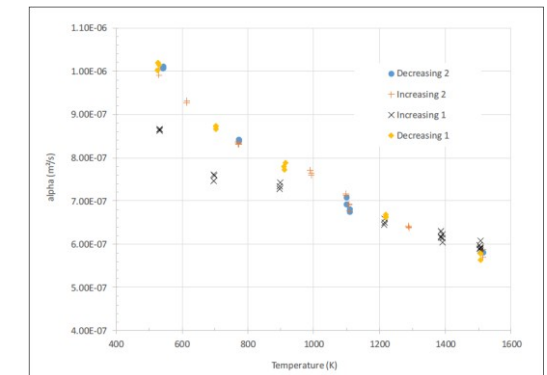
Thermal diffusivity measurements of (U,Am)O 2-x at JRC Karlsruhe
