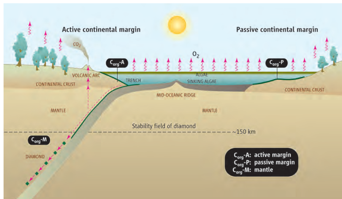
FIGURE 1. PROCESSES CONTROLLING THE FLUX AND ACCUMULATION OF O 2 ON EARTH (FALKOWSKI AND ISOZAKI 2008).
