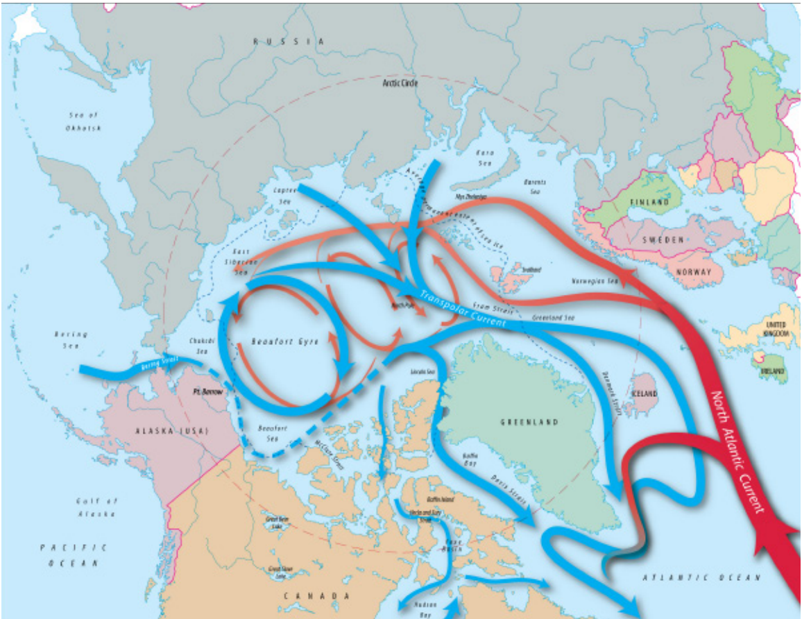
FIGURE 5 The mean pattern of currents in the upper ocean of the Arctic and the subpolar regions. SOURCE: Illustration by Jack Cook ©Woods Hole Oceanographic Institution
