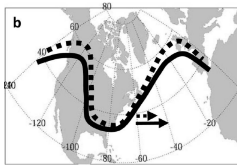
FIGURE 15 This schematic shows ridge elongation (dashed vs. solid) and upper-level wave amplification caused by enhanced warming in Arctic relative to mid-latitudes. Higher amplitude waves progress eastward more slowly, as indicated by arrows. SOURCE: Francis and Vavrus, 2012.
