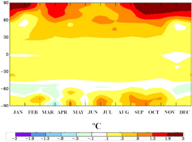
FIGURE 11 This figure shows evidence that the loss of sea ice is already affecting the atmosphere in the autumn and winter. The warmth of 2007-2012, relative to the 1971-2000 “normal”, is shown here as a function of latitude and calendar month. SOURCE: NASA GISS.
