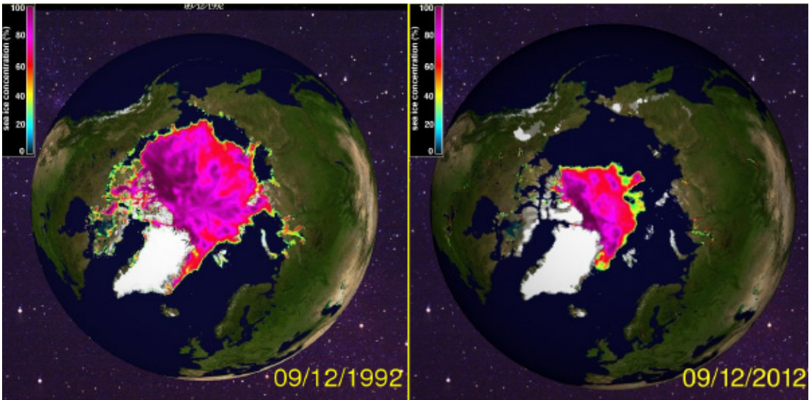
FIGURE 4 A pair of mid-September satellite images from 1992 and 2012 shows the dramatic loss of sea ice in recent decades. SOURCE: University of Illinois, The Cryosphere Today.
