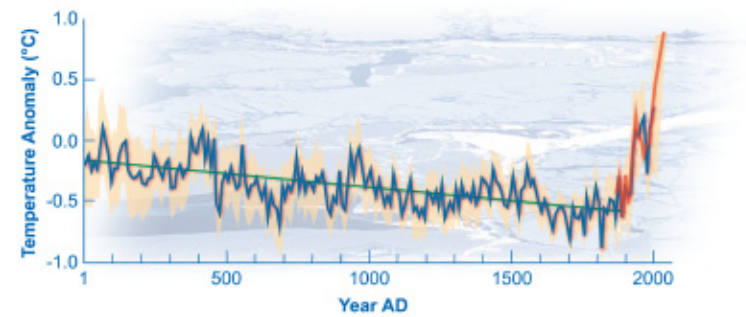
FIGURE 1 A reconstruction of Arctic summer temperatures. The blue line shows estimates of Arctic temperatures over the last 2,000 years, based on proxy records from lake sediments, ice cores and tree rings. The green line shows the long-term cooling trend. The red line shows the recent warming based on actual observations. SOURCE: Kaufman et al., 2009, modified by UCAR.
