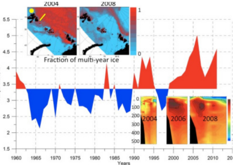
FIGURE 6 Measurements have shown that inflowing Atlantic water has gotten warmer over the past two decades. This image shows concentration of multi-year ice in 2004 and 2008 (two upper insets) and temperature in the Atlantic water core (main graph) measured in Fram Strait (yellow circle, upper left inset) and from transects of different extent (three lower insets) made in September 2004, 2006, and October 2008 at 31E, 80N (location marked by yellow line in the upper left inset). SOURCE: Alexeev et al., 2013.
