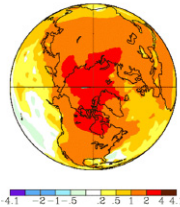
FIGURE 3 Geographic variation in the recent unprecedented rise in Arctic temperature is shown here. This illustrates the poleward increase, or “polar amplification”, of warming. SOURCE: NASA GISS.
