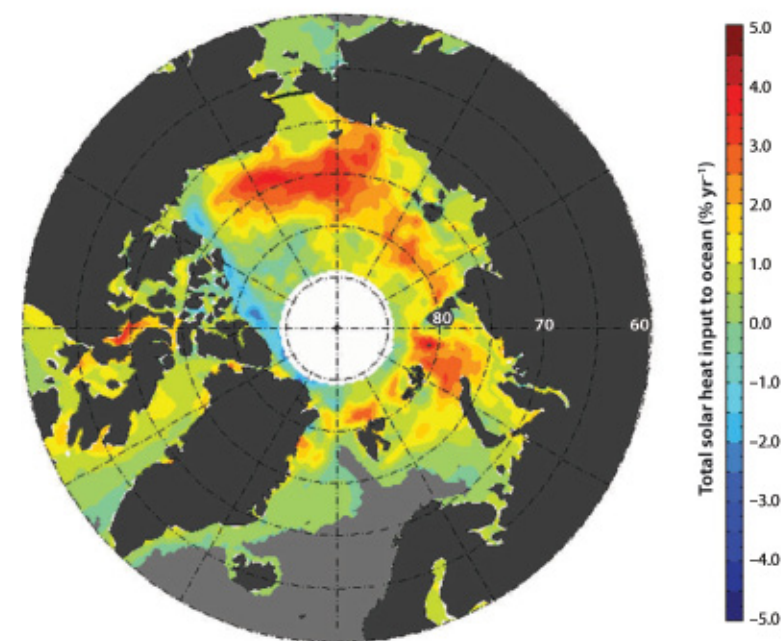
FIGURE 8 Map of the linear trend of annual total solar heat input directly to the ocean. The trend exceeds 2% per year in the orange and red areas, including the Beaufort-Chukchi-East Siberian Sea sector, suggesting a 50% increase over the 26 year period. SOURCE: Perovich and Richter-Menge, 2009.
