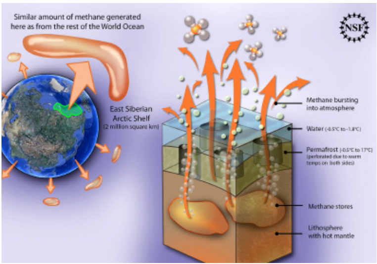
FIGURE 10 The permafrost of the East Siberian Arctic Shelf (an area of about 2 million kilometers squared) is more porous than previously thought. The ocean on top of it and the heat from the mantle below it warm it and make it perforated. This allows methane gas stored under it under pressure to burst into the atmosphere. The amount leaking from this locale is comparable to all the methane from the rest of the world’s oceans put together. Methane is a greenhouse gas more than 30 times more potent than carbon dioxide. SOURCE: Zina Deretsky, National Science Foundation, based on Shakhova et al., 2010.
