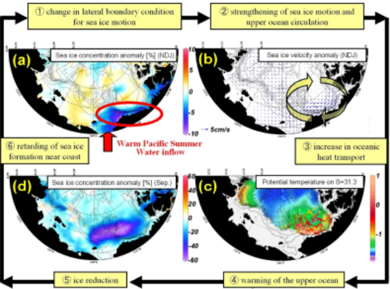
FIGURE 7 Feedback system consisting of (a) Sea ice concentration anomaly for November through January [(1997 Nov.~2003 Jan.) - (1979 Nov.~1997 Jan.)] (b) Sea ice velocity anomaly for November through January [(1997 Nov.~2003 Jan.) - (1979 Nov.~1997 Jan.)] (c) Potential temperature on S=31.3. Background color is climatology from EWG Arctic Ocean Atlas and dotted circles are from 1998–2004. (d) Sea ice concentration anomaly for September [(1998–2003)-(1979–1997)]. SOURCE: Shimada et al., 2006.
