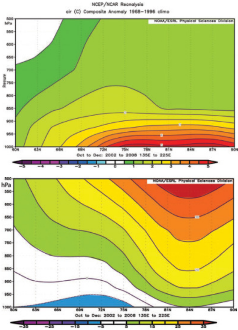
FIGURE 12 This figure shows that Arctic warming is strongest at the ocean surface, and that there has been an increase of elevation (geopotential height) of the pressures in the Arctic atmosphere, as would be expected with warming. (a) The vertical cross-section composite plot of air temperature anomalies ( ^{\circ}\text{C} ) for the section covering East Siberian Sea, Chukchi Sea and Beaufort Sea from Bering Strait to the North Pole for October–December 2002–2008. (b) The vertical cross-section composite plot of geopotential height anomalies (dynamic meters) for the section from Bering Strait to the North Pole for October–December 2002–2008 over the area from Siberian Sea to Beaufort Sea. SOURCE: Overland and Wang, 2010.
