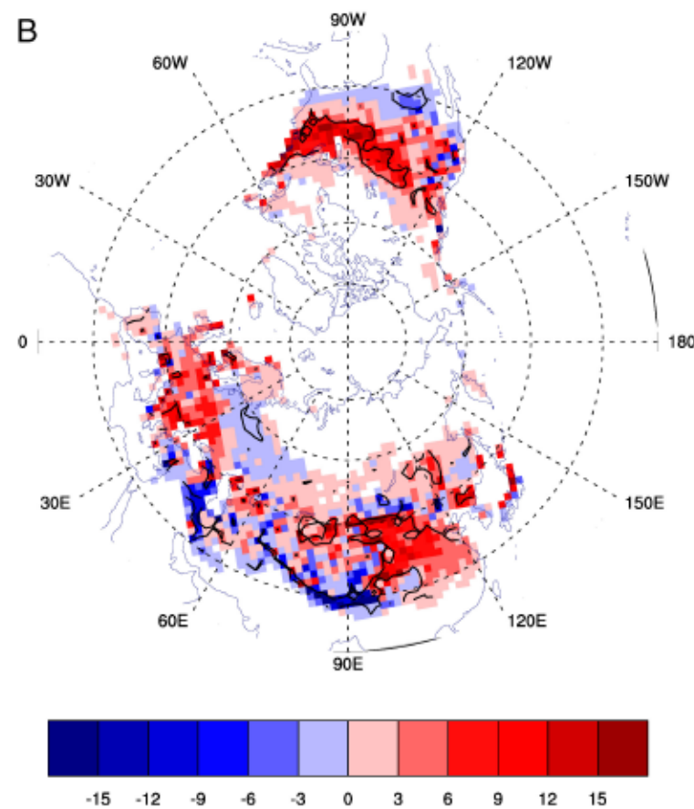
FIGURE 13 Reduced Arctic sea ice extent in autumn is associated with increased winter snow cover in large areas of eastern Asia, central Europe and the northern half of the United States. The image shows linear regression of winter snow cover anomalies (%) on the detrended autumn Arctic sea ice area anomaly (regions within contours denote the regression above 95% confidence level). SOURCE: Liu et al., 2012.
