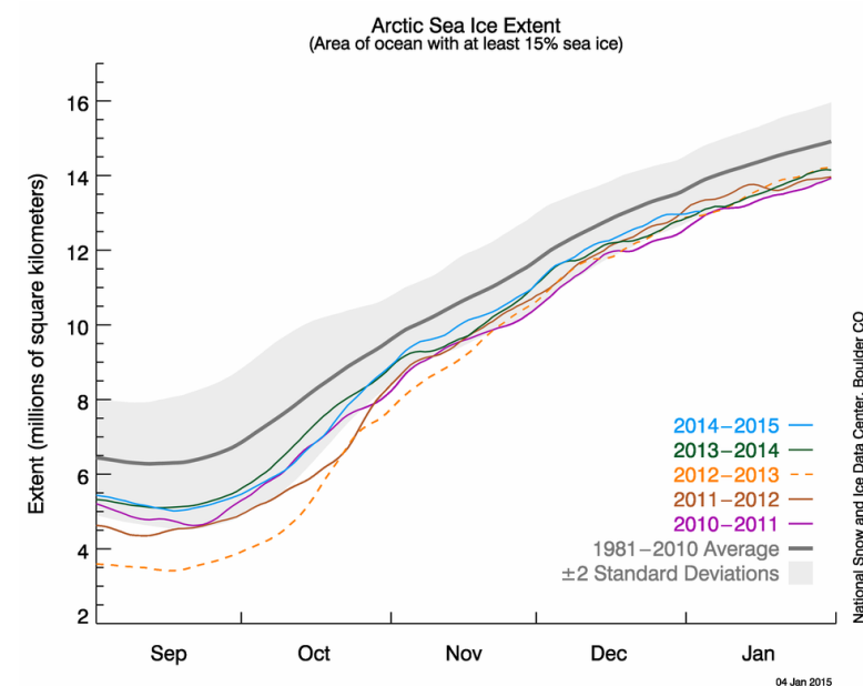
FIGURE 11: Seasonal change in the spatial extent of Arctic sea ice for the past five years compared to the 1981-2010 average (in gray). The minimum in Arctic sea ice generally occurs in September, at the end of the summer warming. Source: Image courtesy of the National Snow and Ice Data Center (NSIDC), University of Colorado, Boulder.
