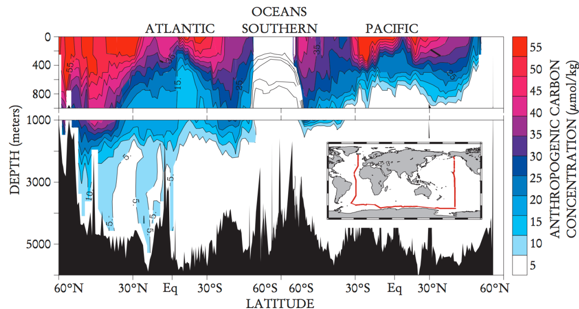
FIGURE 4: Anthropogenic carbon concentration in the ocean along a track shown as a red line in the inset. Of particular note is the penetration of carbon to depths of ~4,000 meters in the high latitudes of the North Atlantic. Source: Reproduced with permission from Sarmiento and Gruber, Physics Today , August 2002, American Institute of Physics.
