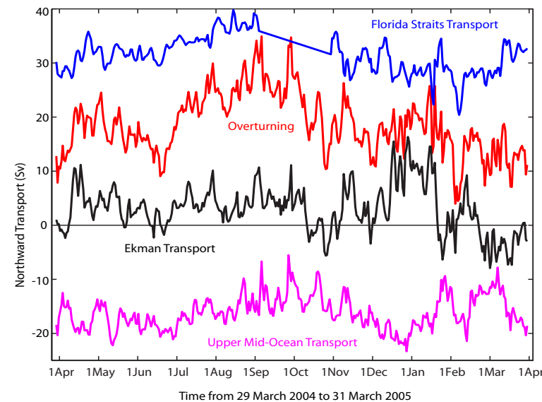
FIGURE 6: Time series of the meridional overturning circulation at 26°N, measured from the Rapid array. The meridional overturning circulation is the sum of the Gulf Stream transport through the Florida Straits, the wind-driven Ekman current, and the midocean geostrophic transport. Source: Cunningham et al., 2007.
