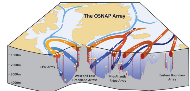
FIGURE 12: Schematic of the Overturning in the Subpolar North Atlantic Program (OSNAP) observing system, deployed in the summer of 2014. Arrays of current meters span the boundary currents in the Labrador, Irminger and Iceland Seas, as well as in the Rockall Trough. Deep arrays have been deployed on both sides of the Reykjanes Ridge. The observing system will allow for monthly estimates of the overturning circulation, as well as the flux of heat and freshwater across the array. Subsurface floats deployed in the deep waters for the purpose of tracing water mass pathways are also part of the OSNAP program, as are gliders that patrol the waters above the Hatton/Rockall Bank. A contribution to this observing system from the People's Republic of China is expected to be made in the summer of 2015. Source: Image courtesy of Overturning in the Subpolar North Atlantic Program (OSNAP). Schematic credit: Penny Holliday (National Environmental Research Council, U.K.)
