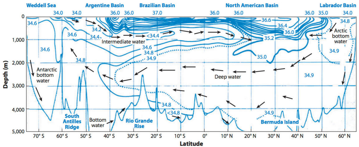
FIGURE 2: Meridional cross-section of salinity in the western Atlantic Ocean constructed from measurements during the German Atlantic expeditions from 1925-1927. Source: Lozier, 2012. Adapted from Tchernia, 1980, where it was reprinted from Merz, 1925.
