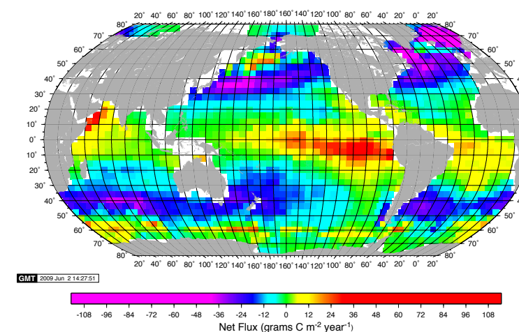
FIGURE 5: The annual flux of CO 2 across the air-sea interface, produced from surface water measurements taken since 1970. Negative values indicate a flux of CO 2 into the ocean; positive values indicate a CO 2 flux out. Note the large negative values in the northern North Atlantic. Source: Takahashi et al., 2009.
