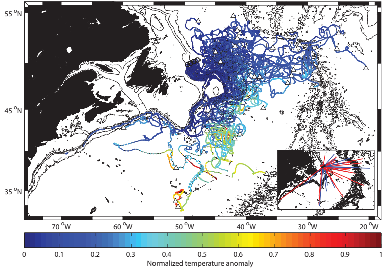
FIGURE 8: Trajectories of 40 acoustically tracked floats released at 700 and 1,500m in the Deep Western Boundary Current in the Labrador Sea and followed for two years. Daily float positions are indicated with color-coded dots, where the color denotes the change in temperature along the float's path. Dashed lines indicate missing track. The inset shows the two-year displacement vectors for the 700 m (red) and 1,500 m (blue) floats. Source: Bower et al., 2008.
