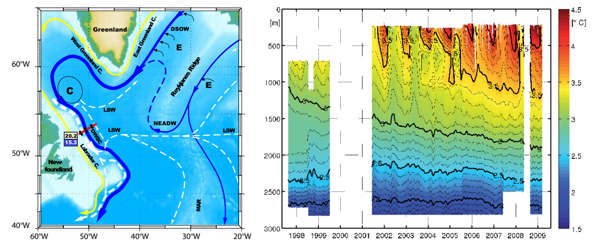
FIGURE 10: (left) The Labrador Sea in the North Atlantic with the site of a long-term mooring array situated in the Deep Western Boundary Current denoted by the red line. (right) The evolution of the temperature field in the center of Deep Western Boundary Current. Note the warming of the waters from near the surface down to ~2,000 m in the latter part of the record. Source: Fischer et al., 2010.
