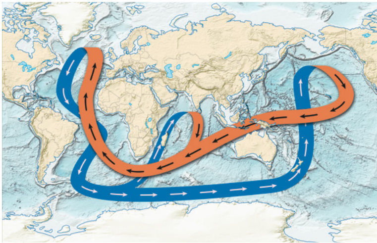
FIGURE 1: Schematic of the ocean conveyor belt. Arrows indicate direction of flow. Orange, the warm, shallow waters of the upper limb of the conveyor belt; blue, the cold, deep waters of the deep limb. Source: Lozier, 2010. Used with permission from Joe LeMonnier.
