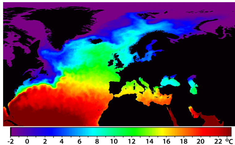
FIGURE 9: Sea surface temperature for the North Atlantic in January of 2008, measured from satellites. Source: Image courtesy of Valborg Byfield, National Oceanography Center, Data from OSTIA.
