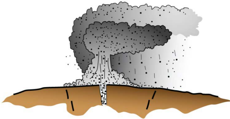
Stage 2—Beginning of column collapse
