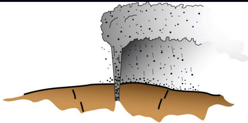
Stage 1—Ash fall
