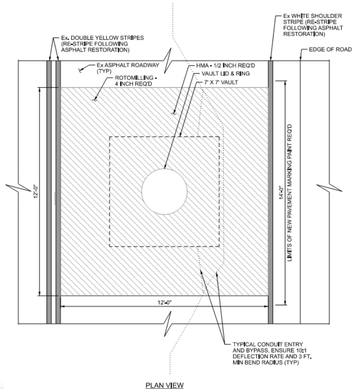
PLAN VIEW
