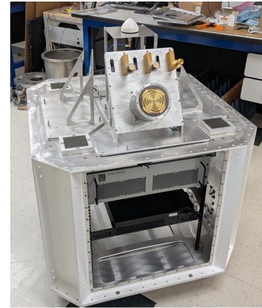
The ASM-2 enclosure (L-above) is manufactured locally (in VA). ASM-2 assembly proceeding last week (R-above)
