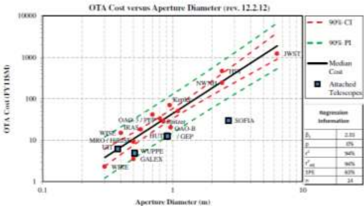
Telescope cost as a function of aperture diameter for space-based telescopes (Figure credit: SPIE)
